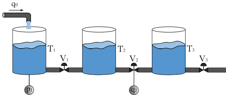
Figure 8: Diagram of the three-tank system.
