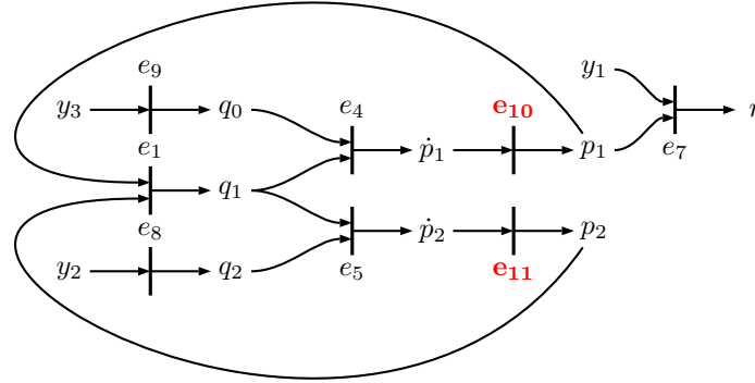
Figure 13: Residual r_2 , sequential residual generator in integral causality based on mso \mathcal{M}_2 .
